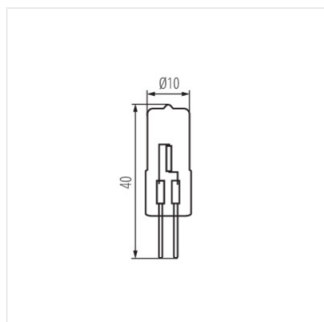
JC-20W GY6.35; 35W GY6.35; 50W GY6.35
