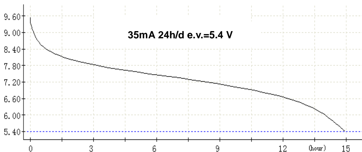
Chart 1. Discharge diagram
