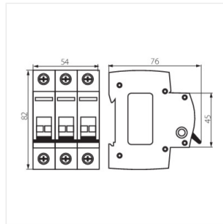
KMI-3/100A
