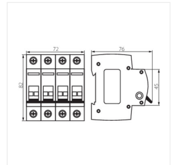
KMI-4/100A
