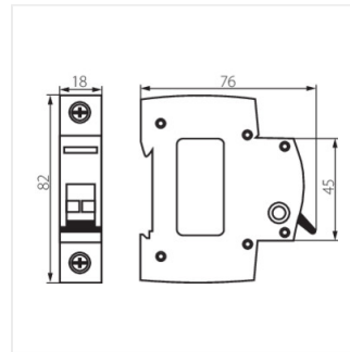
KMI-1/63A
